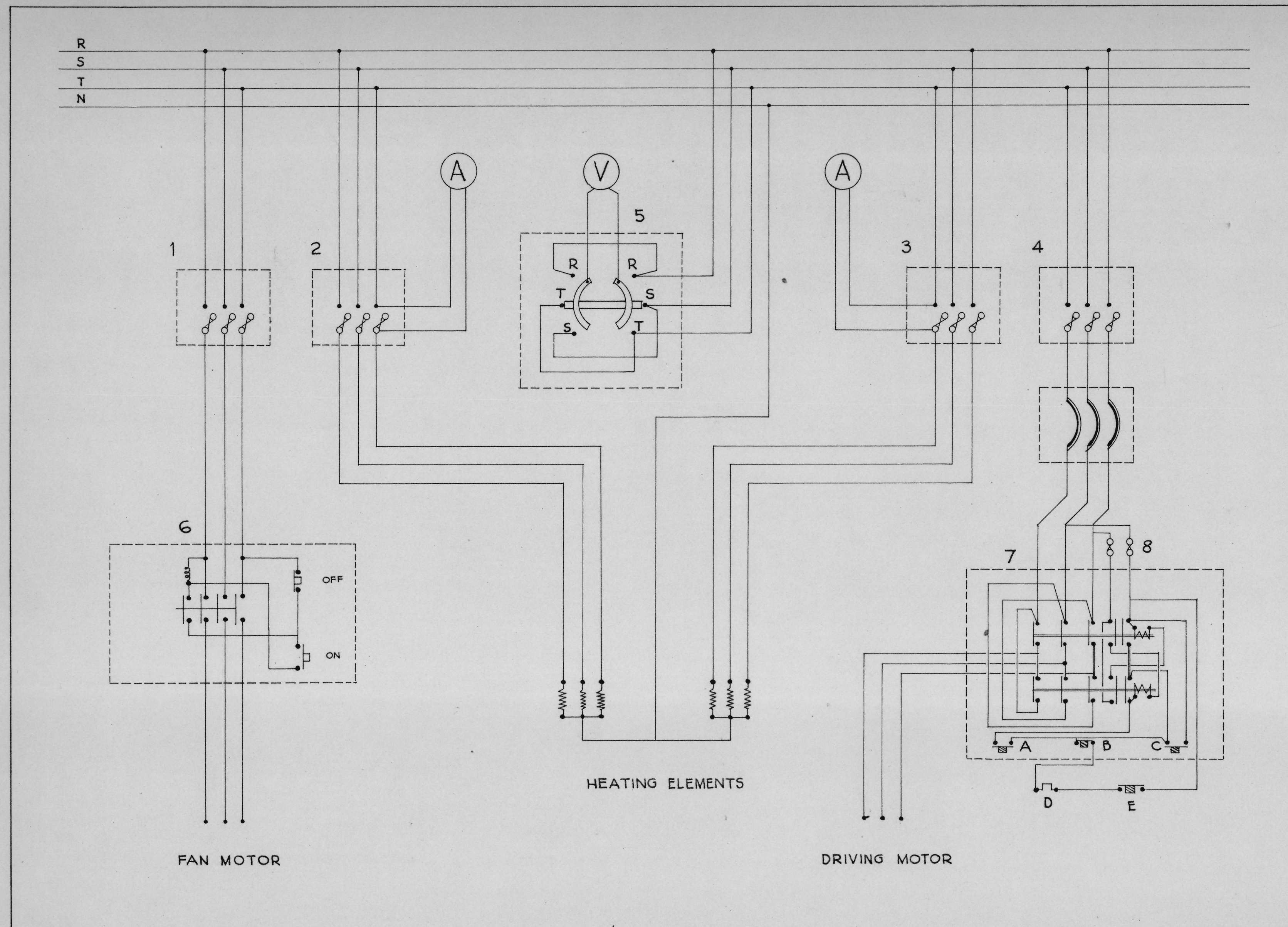
CONNECTION DIAGRAM FOR CONTROL AND HEATING OF CALENDER
