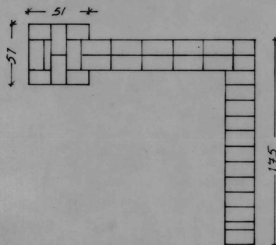
PLAN COURSES-1-3
