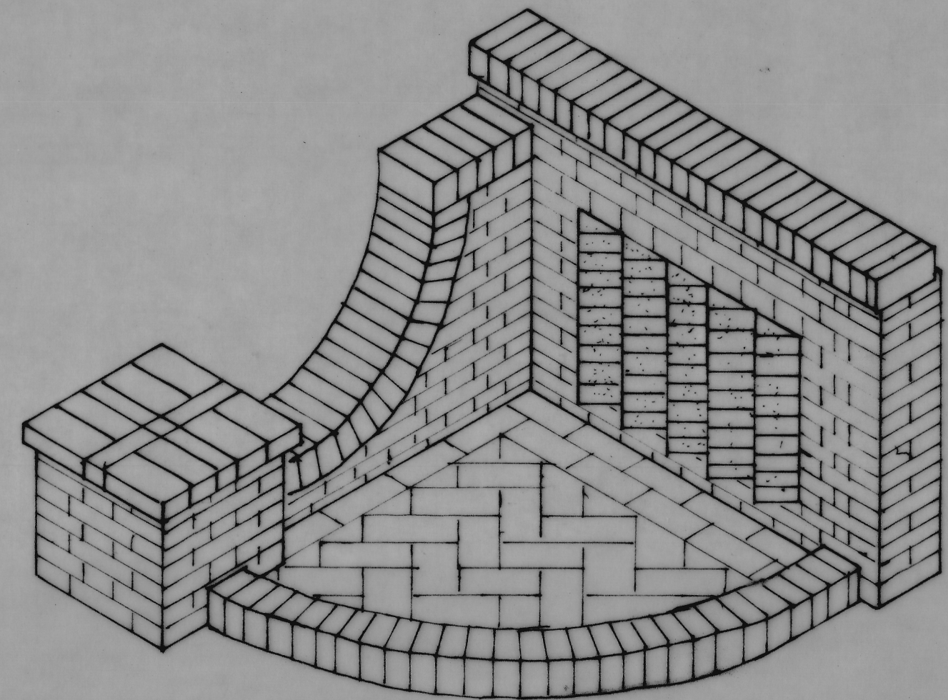
ISOMETRIC SKETCH
