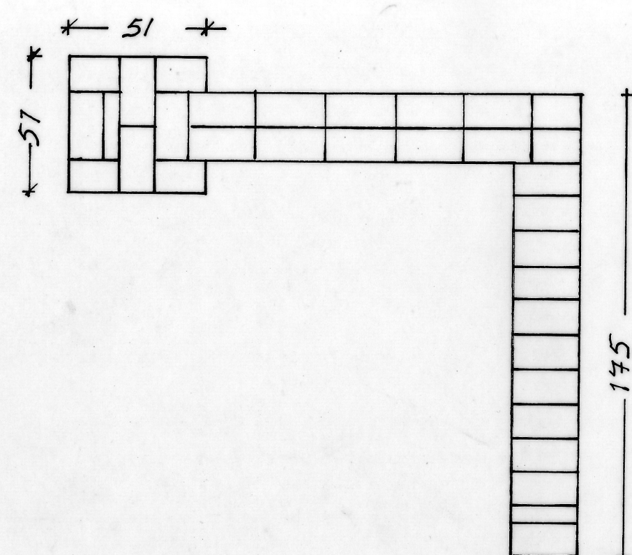
PLAN COURSES-1-3
