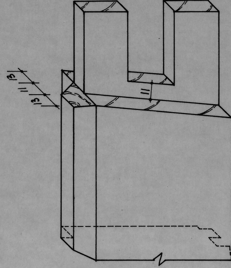
DETAIL OF TENON A
