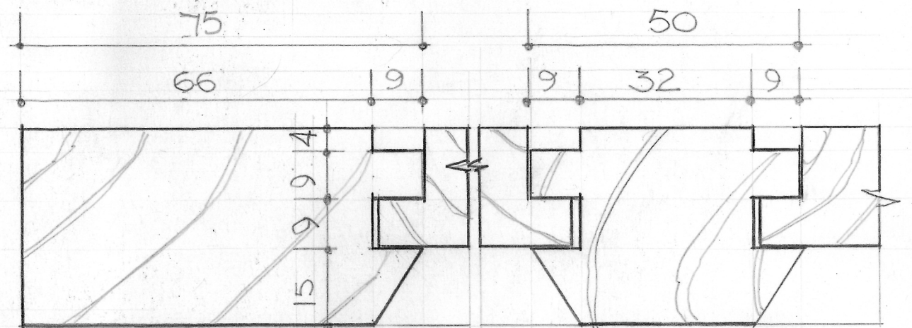
DETAIL OF BOTTOM PORTION SCALE 1:1
