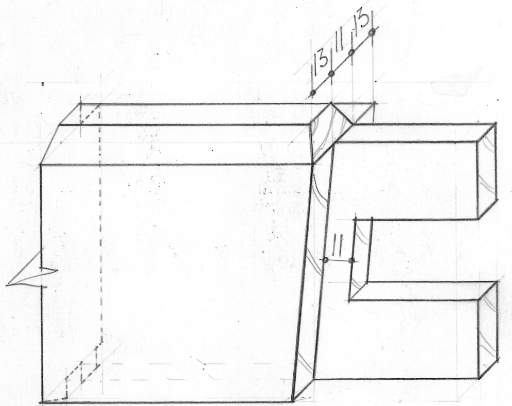
DETAIL OF TENON A SCALE 3:5
