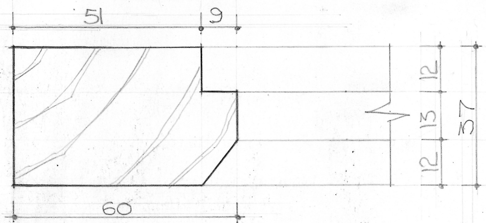
DETAIL OF TOP PORTION
