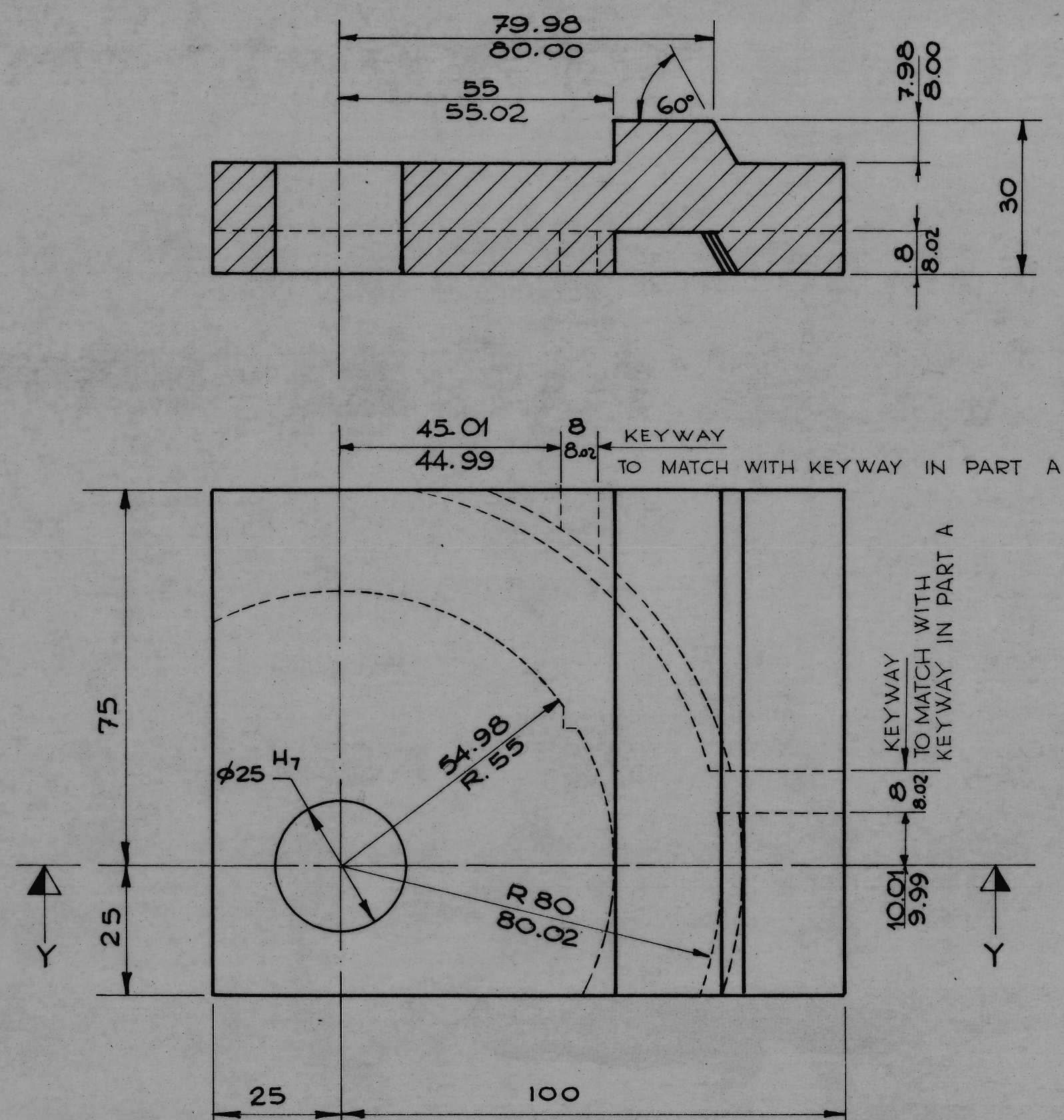
SECTION Y-Y
