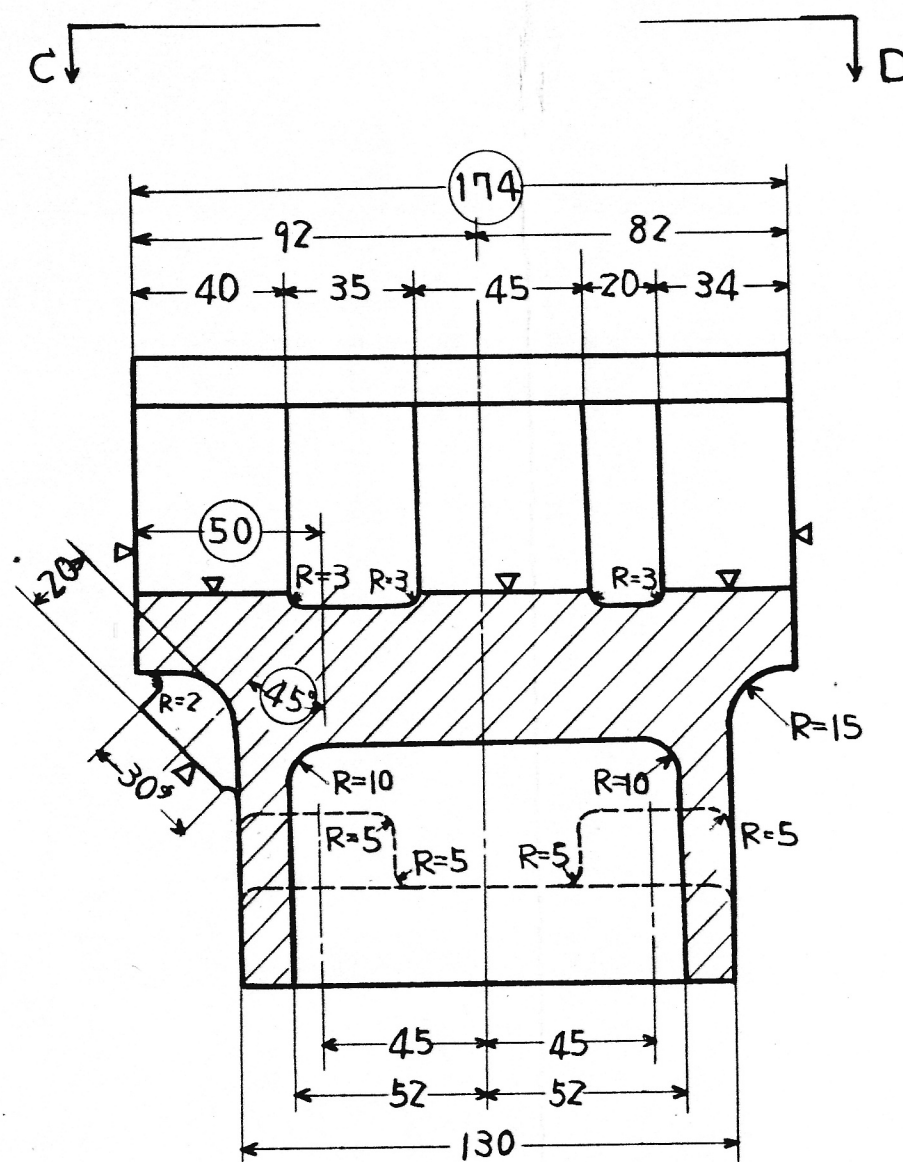
VIEW C-D
