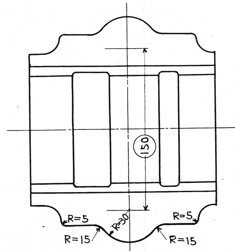
VIEW C-D
